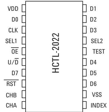
PINOUT C
